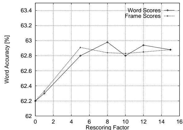
Figure 5: Word scores vs. frame scores.
