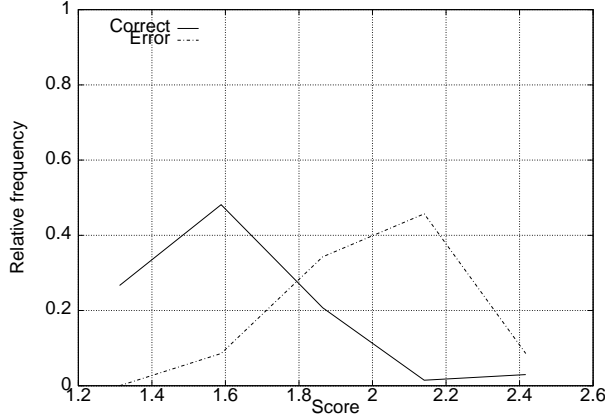
Figure 2: The word denke exhibits two well separated distributions. Scores are frame-based.
