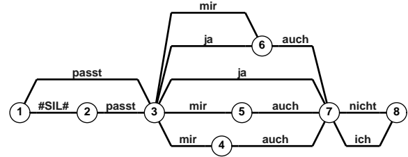
Figure 4: Example of a word graph.
